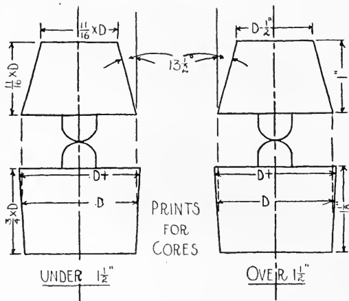
FIG. 539. CORE-PRINT DETAIL.
